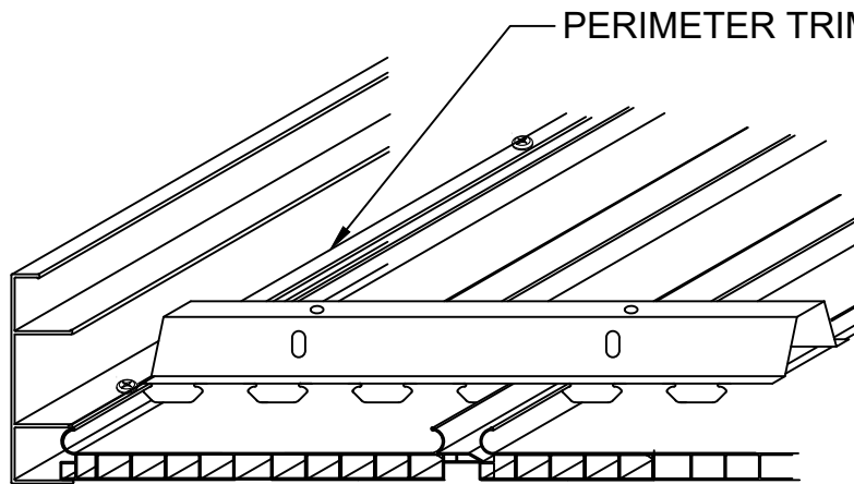
A SIDE INSTALLATION
