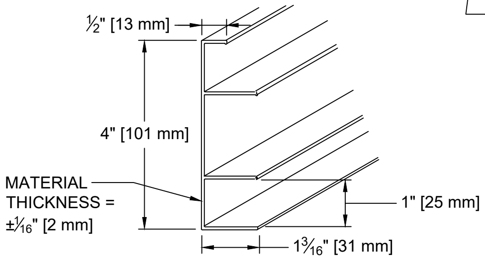
C #872 PERIMETER TRIM CROSS-SECTION
