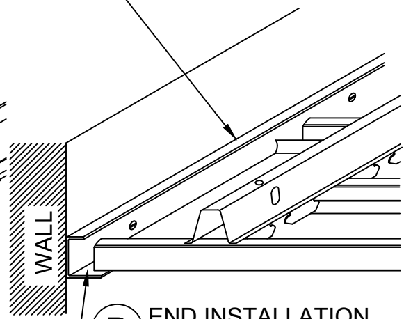
B END INSTALLATION
