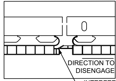
LATCH DETAIL (SHOWN CLOSED)
