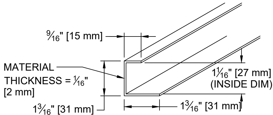
C #870 PERIMETER TRIM CROSS-SECTION
