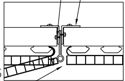
HINGE DETAIL (SHOWN CLOSED)
