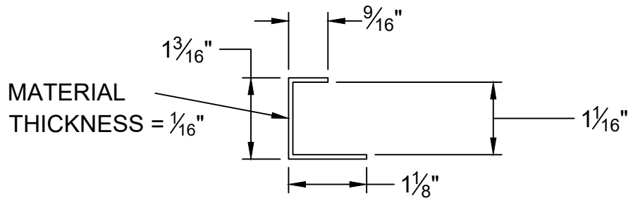
C #870 PERIMETER TRIM CROSS-SECTION
