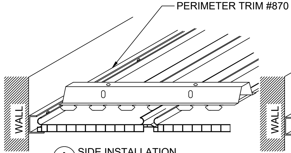
A SIDE INSTALLATION
