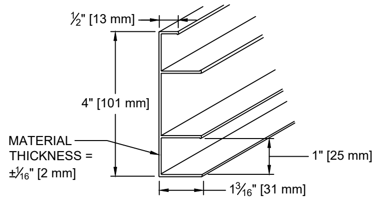
C #872 PERIMETER TRIM CROSS-SECTION
