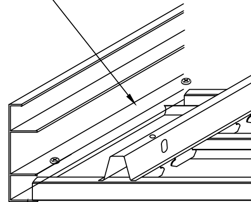
C #872 PERIMETER TRIM CROSS-SECTION
