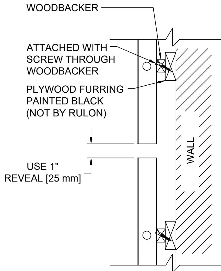
WALL SECTION
