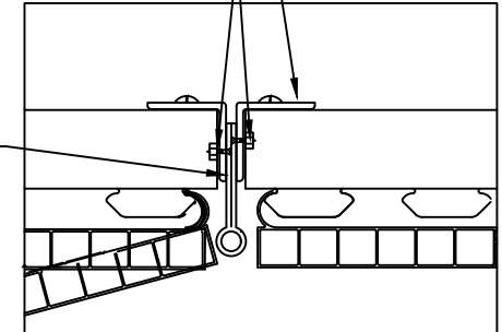
HINGE DETAIL (SHOWN CLOSED)
