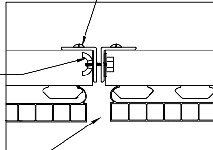
LATCH DETAIL (SHOWN CLOSED)
