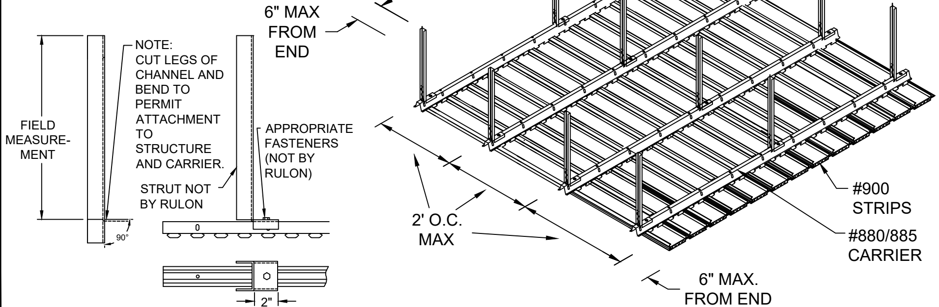
TYPICAL STRUT
