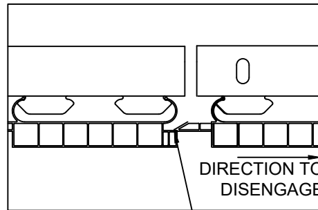
LATCH DETAIL (SHOWN CLOSED)
