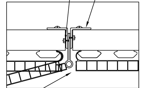
HINGE DETAIL (SHOWN CLOSED)
