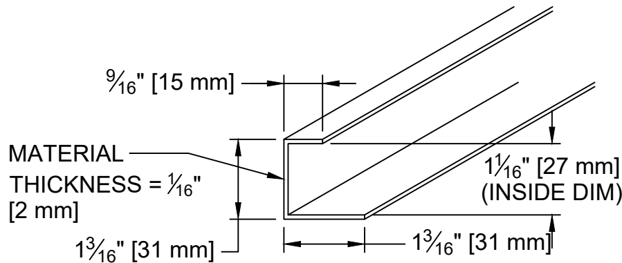
C #870 PERIMETER TRIM CROSS-SECTION
