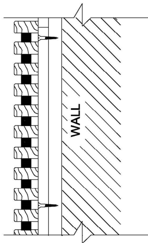
WALL SECTION
